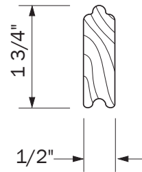
Wood Slat Profile (view from the side)
